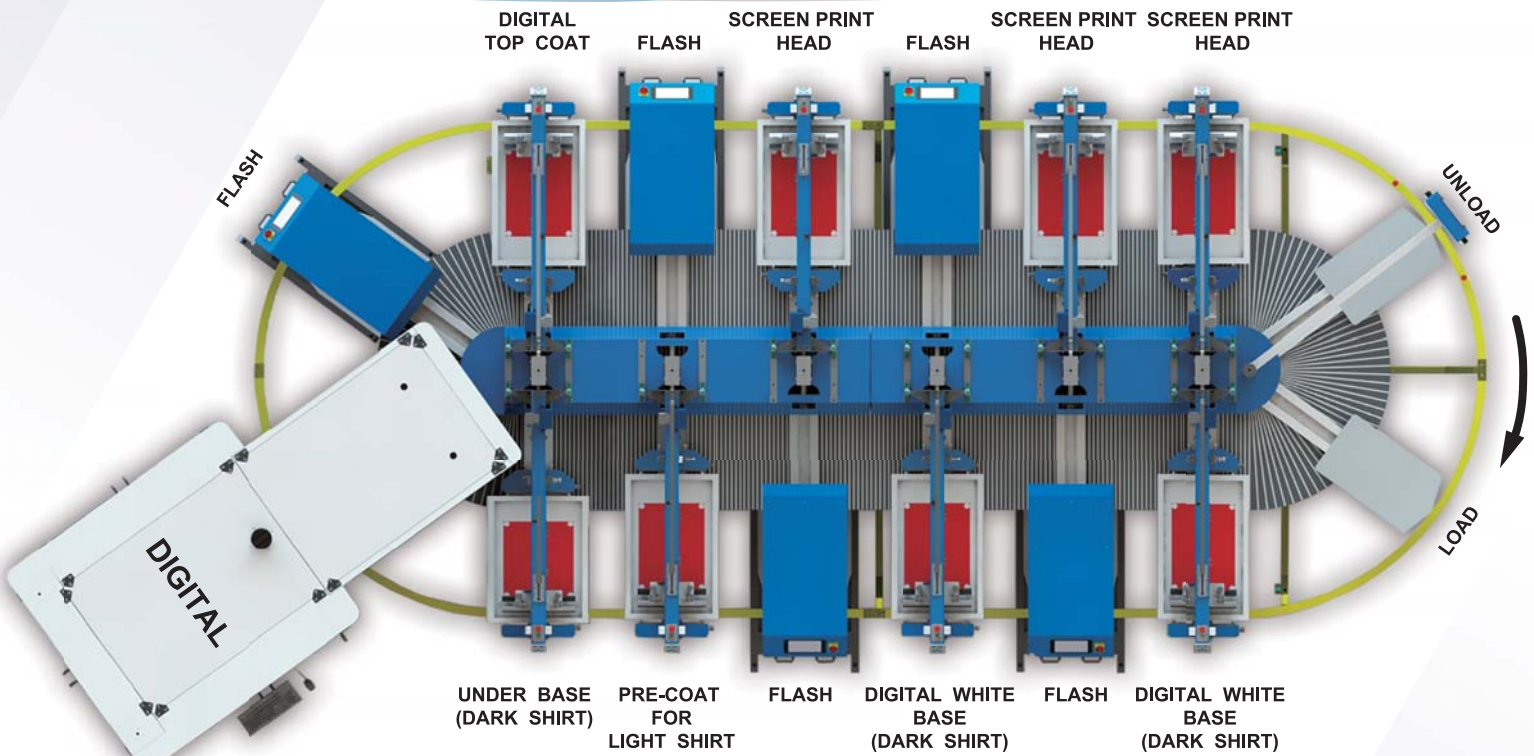
ADELCO HYBRID & OVAL SCREEN / DIGITAL SET-UP EXAMPLE
